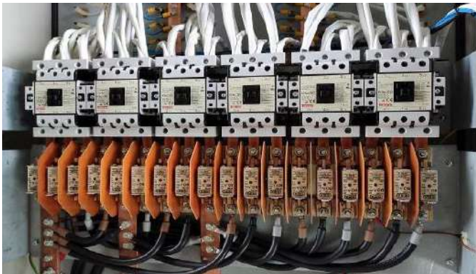
Figure 4. Main 6 contactors with connected set of heating elements
