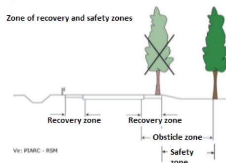
Figure 3. Safe road principle – the width and length of the safety zone depend on the type of roadway and vary from country to country
