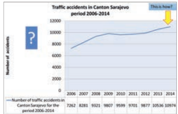
Figure 5. Number of traffic accident in Canton Sarajevo for the period 2006-2014, Federal Ministry of Interior
