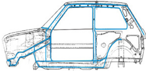
Figure 10. Places of application of structural adhesives on the body of a Koral vehicle
