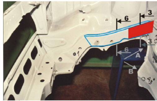
Figure 4 Sensitive zones on the frontal skeleton
