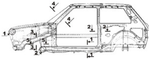
Figure 2. Supporting construction
