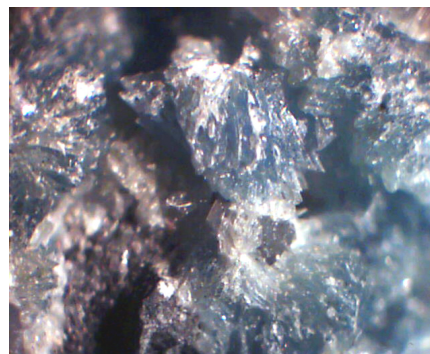
Figure 2 Crystal druse of vauxite
