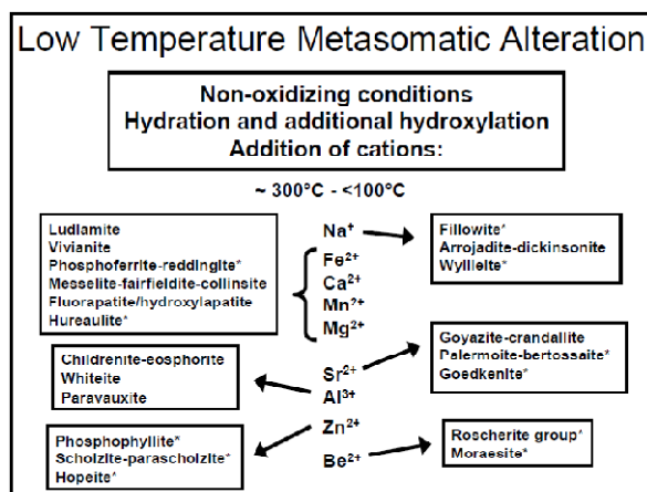
Figure 5 Scheme of the low-temperature phosphate formation in reducing conditions [22].
