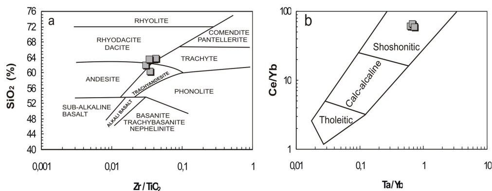
Figure 3. a) \text{SiO}_2 - \text{Zr}/\text{TiO}_2 diagram [10] and b) \text{Ce}/\text{Yb} - \text{Ta}/\text{Yb} diagram for classification of Tertiary volcanics from the Maglaj environment
