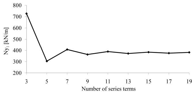
Figure 9 Convergence of normal force N_{y1} by number of series terms for discretization with 12 strips
