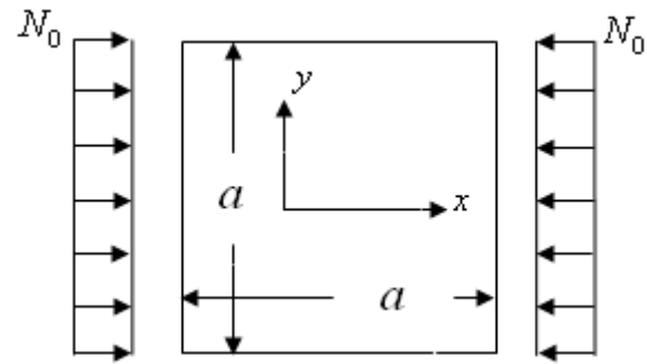
Figure 2. Square plate subjected to uniaxial compression
