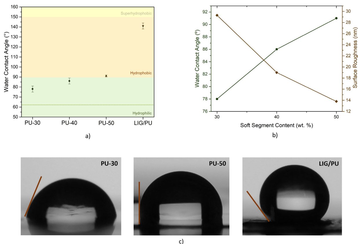
Figure 3. a) Static water contact angles of pure PUs and average WCA of LIG/PUs; b) Water contact angles and surface roughness with varying SSC in PU matrix; and c) From hydrophilic to bordering superhydrophobic surfaces.
