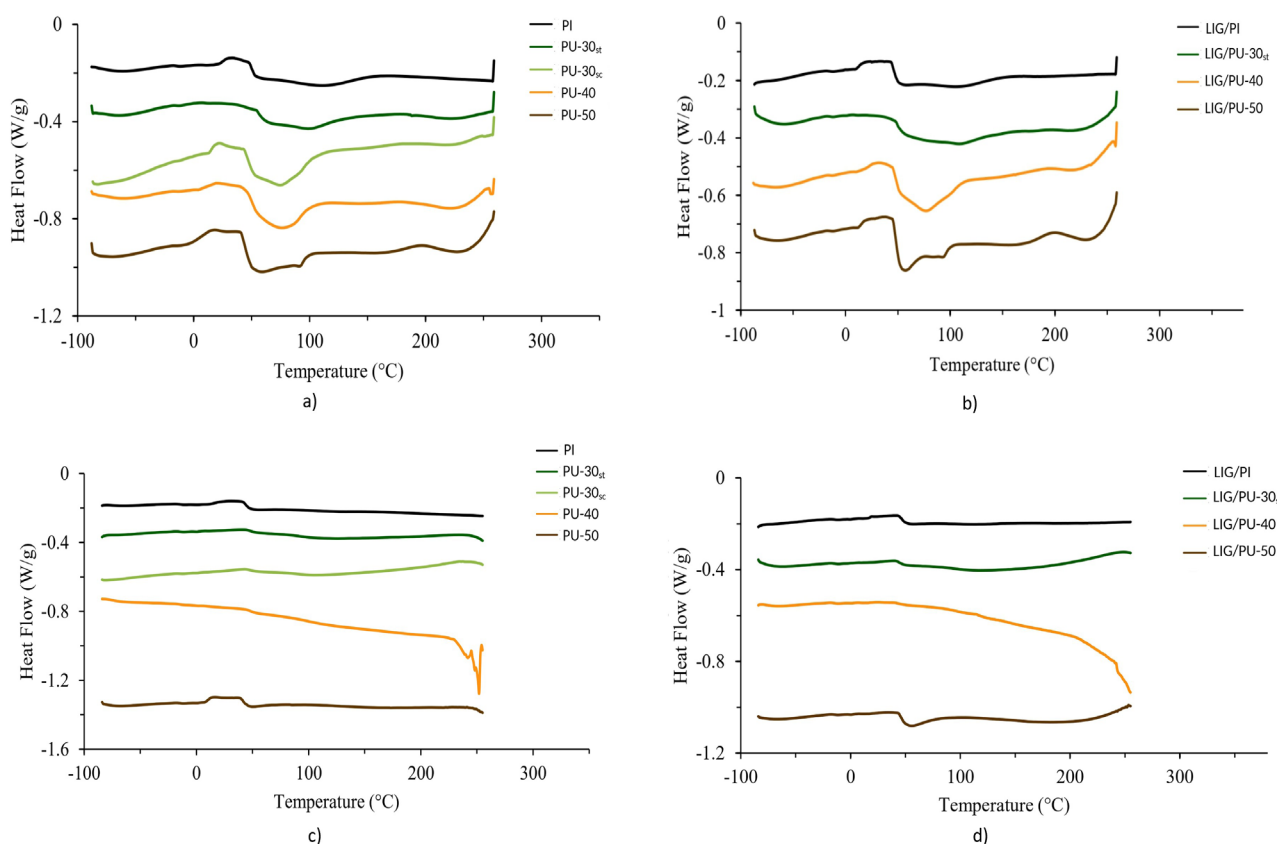
Figure 4. DSC thermograms: a), b) for the C_1 scan, and c), d) for the C_3 scan. The samples are denoted in the figure..
