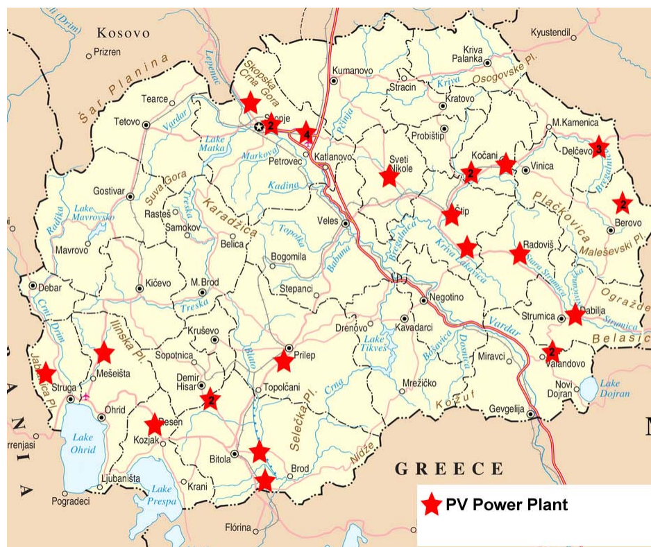
Figure 1. Geographical location of photovoltaic power plants in the Republic of Macedonia. (Derivative work. Map based on [31])
