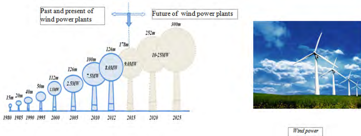
Figure 7. Historical development of wind power plants size and the future development scenario
