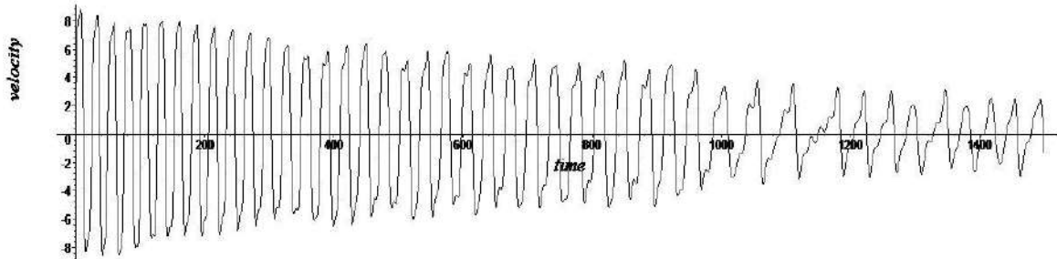
Figure 6. Velocity of the Duffing oscillator for 2.7 \leq F_f \leq 3.0 .
