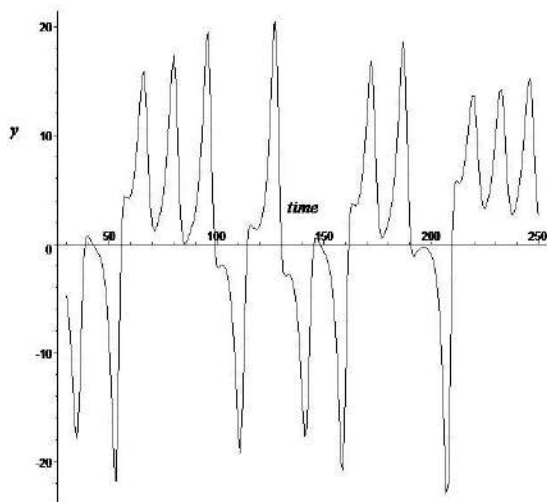
Figure 9. y(t) for -10 \leq F_f \leq 0 .
