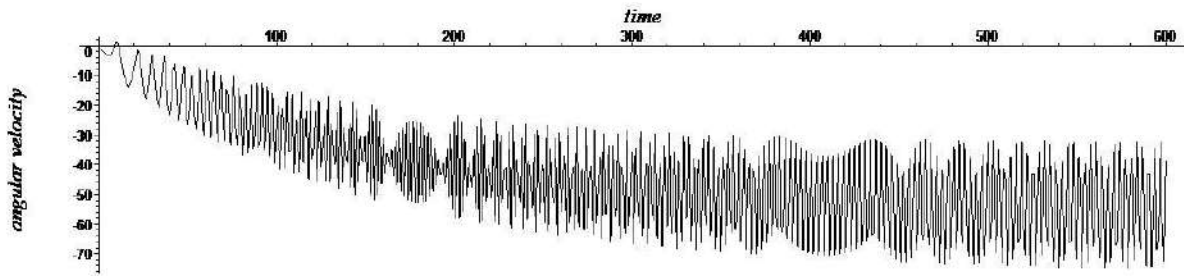
Figure 3. Angular velocity of the first pendulum for -70 \leq F_f \leq -63 (second realization of a series of random numbers). After a long enough period approximate periodicity appears.
