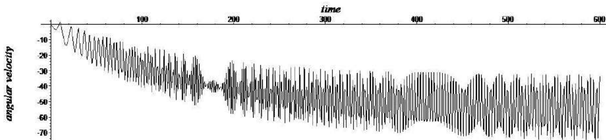
Figure 2. Angular velocity of the first pendulum for -70 \leq F_f \leq -63 .
