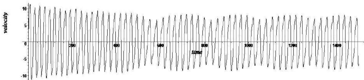
Figure 8. Velocity of the Duffing oscillator for 10.8 \leq F_f \leq 12.0 .
