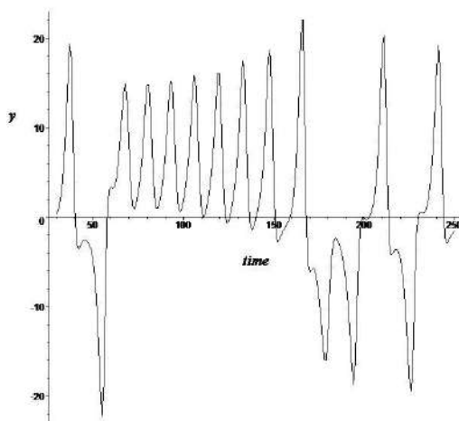
Figure 11. y(t) for 10 \leq F_f \leq 20 .
