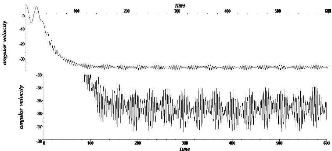
Figure 5. Angular velocity of the Thacker oscillator for -30 \leq F_f \leq -27 .
