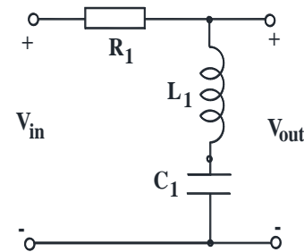
Fig. 1: RLC circuit of notch filter
