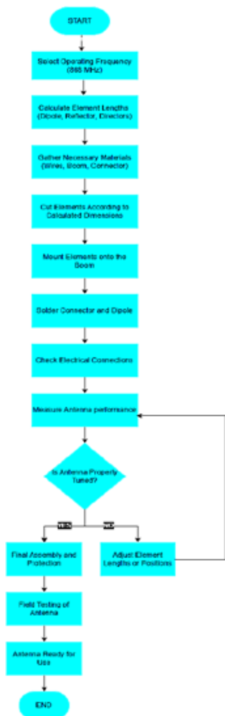
Figure 2. Flowchart of Yagi antenna construction process
