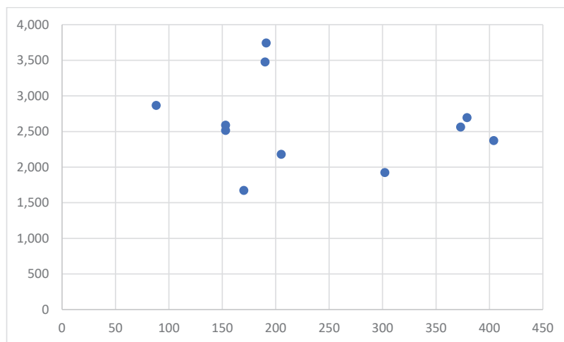
Chart 3. Scattering curve (Author)
